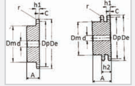
TEK SIRA - SIMPLEX
