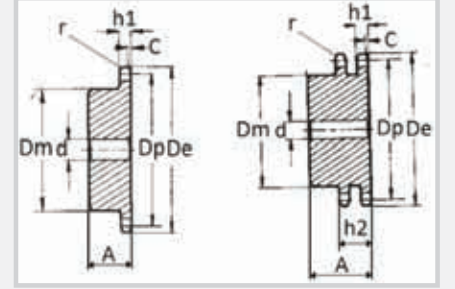
TEK SIRA - SIMPLEX
